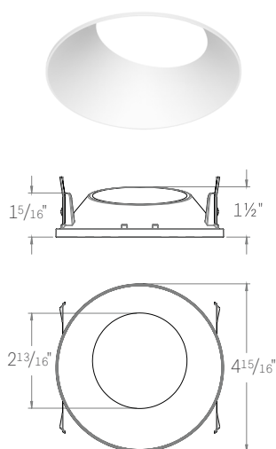
ED5-RATL ROUND ADJUSTABLE TRIMLESS Adjustable trim styles for use with adjustable SAIC models only.
